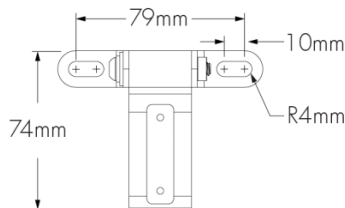
UMP - Mounting hole pattern
